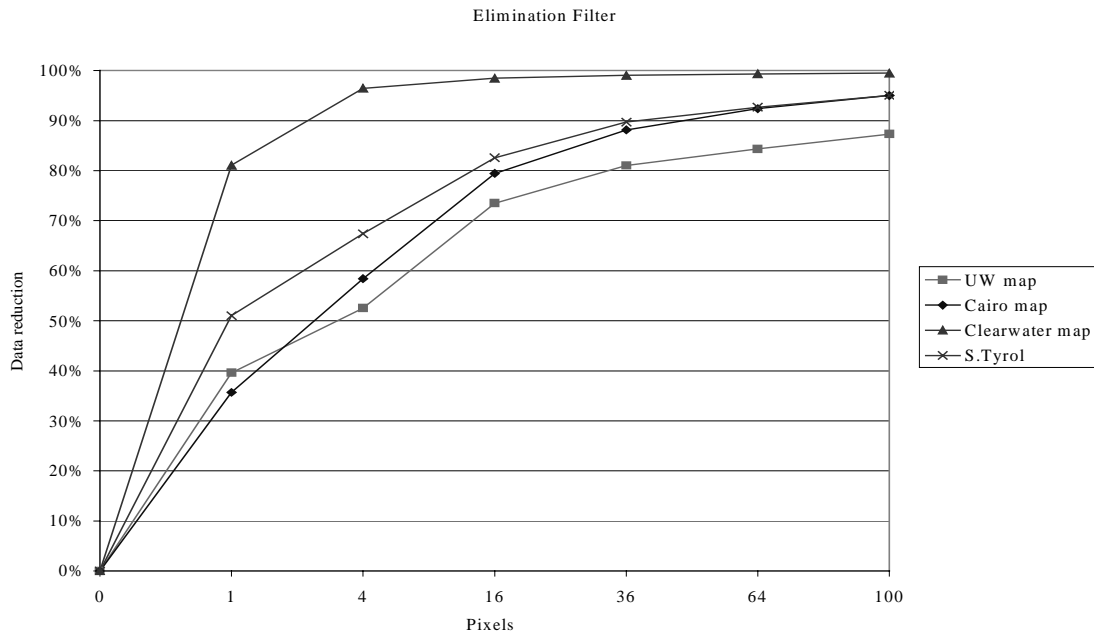
Figure 17. Elimination filter experiment results
