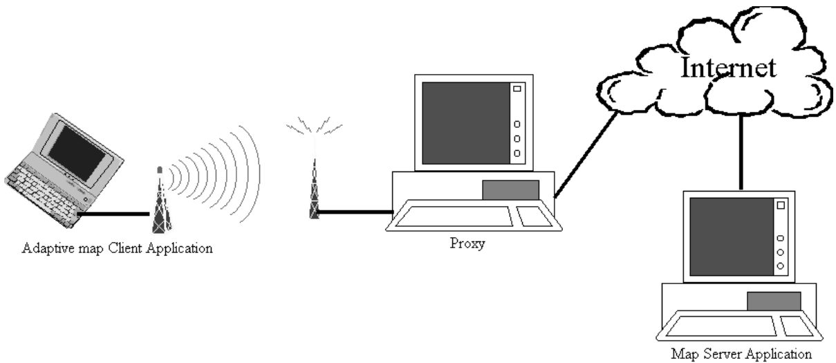
Figure 3. Client-proxy-server model
